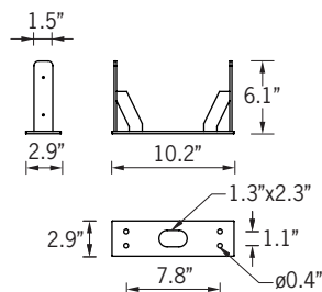
Mounting Detail
