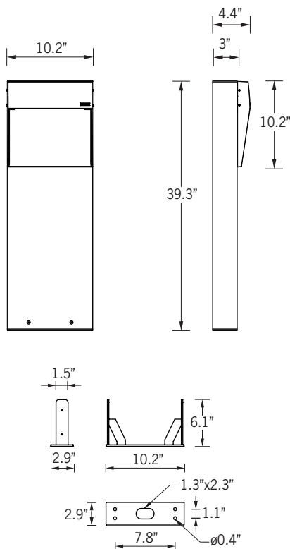
Mounting Detail
