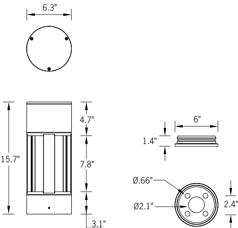
Mounting Detail
