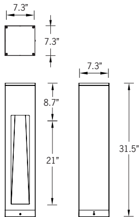
Mounting Detail
