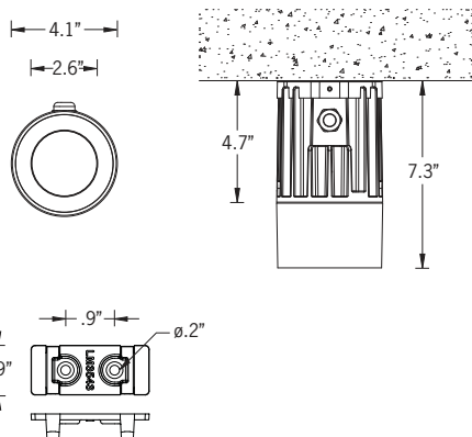
Mounting Detail
