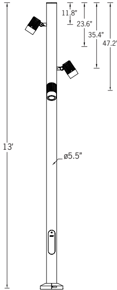
Floodlight Detail
