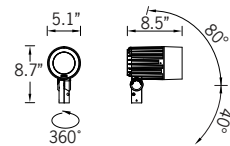
Floodlight Detail
