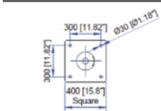
Mounting Detail
