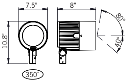
Floodlight Detail
