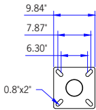
Mounting Detail
