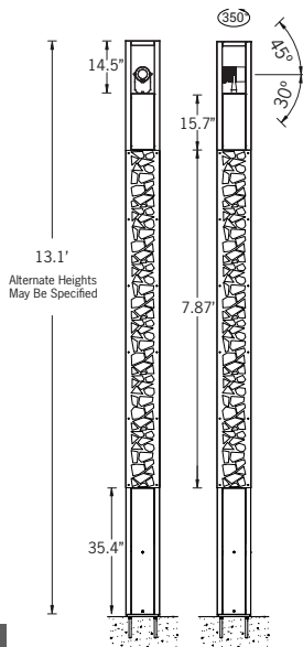
Mounting Detail
