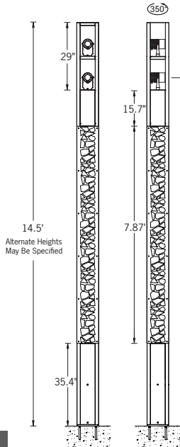
Mounting Detail
