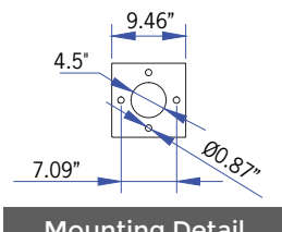
Mounting Detail
