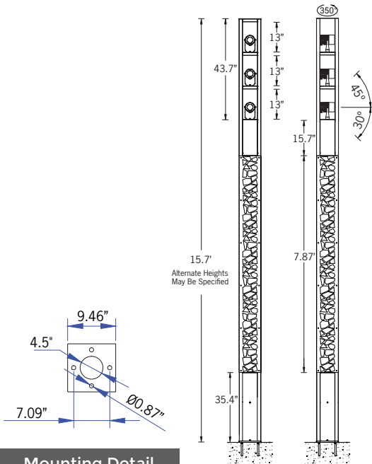
Mounting Detail
