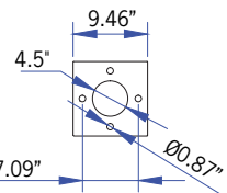
Mounting Detail
