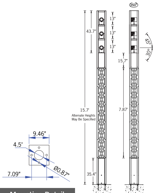
Mounting Detail
