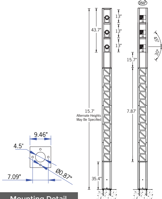
Mounting Detail
