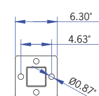
Mounting Detail
