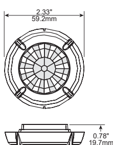
FSP-L3 dimensions
