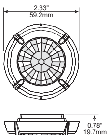
FSP-L3 dimensions
