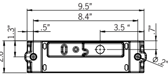
Mounting Detail
