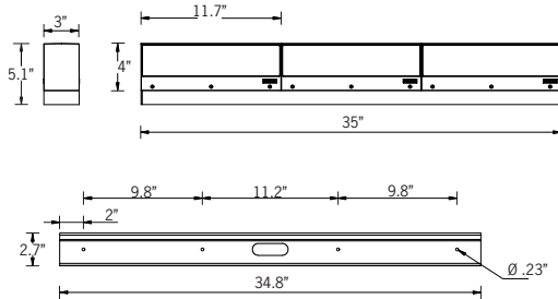
Mounting Detail
