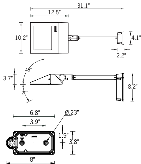
Mounting Detail
